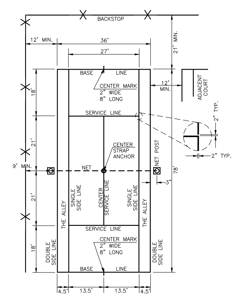
TENNIS COURT STRIPPING LAYOUT
