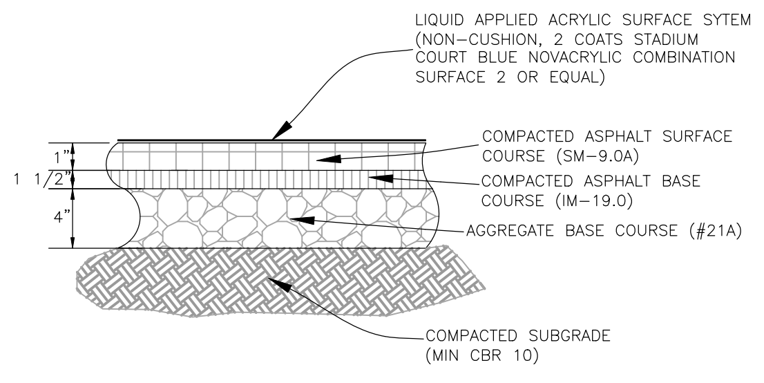
TENNIS & PICKLE BALL COURT SECTION
