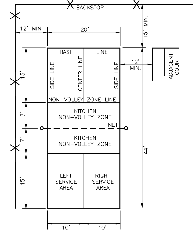
PICKLE BALL COURT STRIPPING LAYOUT
